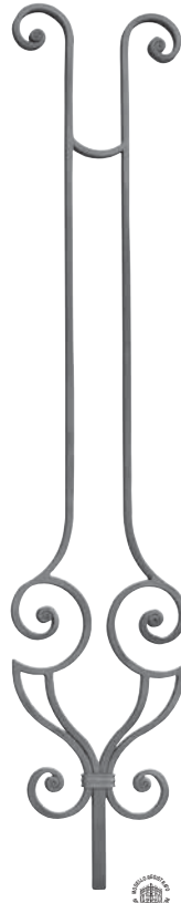
Art. GDI48/1 \Phi 14 \times 14 mm H 1000 mm L 205 mm
